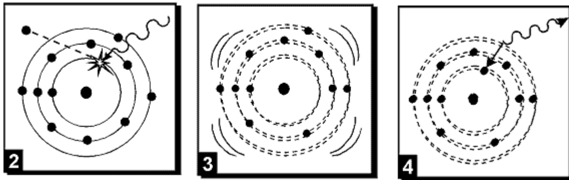
Figure 15—X-Ray Energies
